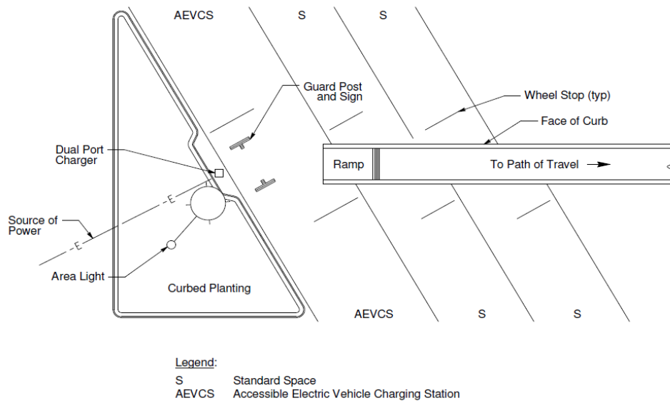
Figure 3: Example of First Two EVCS in Existing Parking Facility
