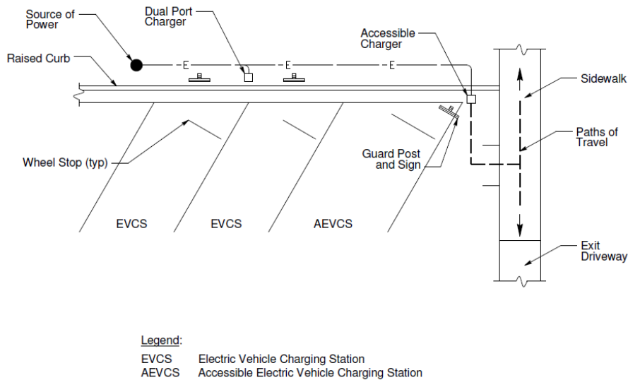
Figure 4: Example of First Two EVCS in Existing Parking Facility
