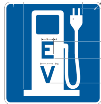
Figure 7 - D9-11b (Alternate) Source: CA MUTCD
