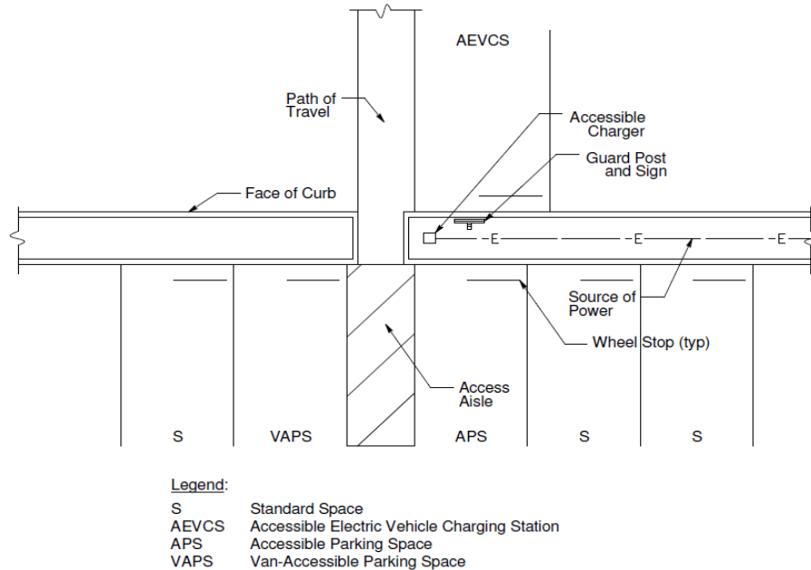
Figure 2: Example of First EVCS in Existing Parking Facility
